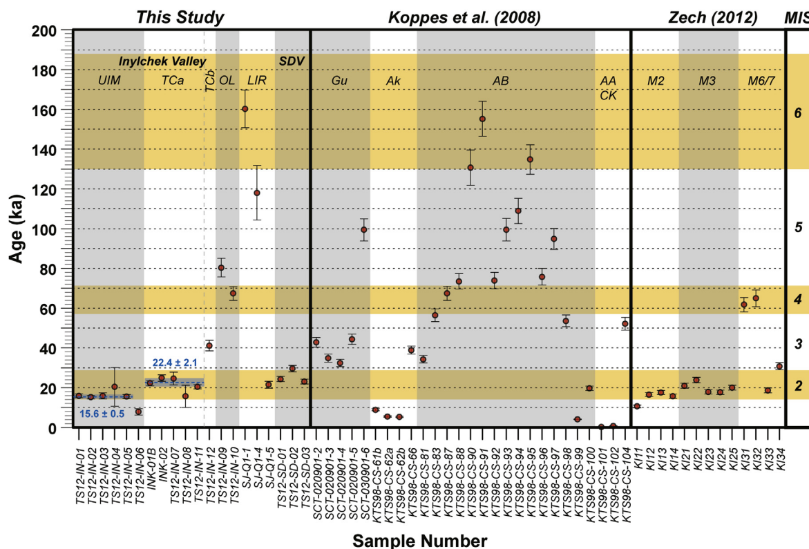
Fig. 5. Comparison of apparent ^{10}\text{Be} exposure ages from Inylchek/Sary-Dzaz valleys with recalculated Koppes et al. (2008) and Zech (2012) apparent ^{10}\text{Be} exposure ages (Table 1 and S1 in the appendix). Approximate MIS boundaries in gold from Lisiecki and Raymo (2005). Site abbreviations: UIM = Upper Inylchek moraines; TC = Terminal moraine complex, TCa = main ridge, TCB = ridge outboard of main ridge; OL = Older lateral moraine; LIR = Lower Inylchek remnant; SDV = Sary-Dzaz Valley. Koppes et al. (2008) site abbreviations: Gu = Gulbel; Ak = Aksai; AB = Ala Bash; AA = Ala Archa; CK = Chor Kyrchak. Blue dashed lines and shading around the UIM and TCa samples indicate inverse relative-error-weighted means for each landform. TS12-IN-08 is included in the TCa weighted mean. Excluding that sample does not change the mean value or uncertainty significantly ( 22.5 \pm 2.0 ka).
