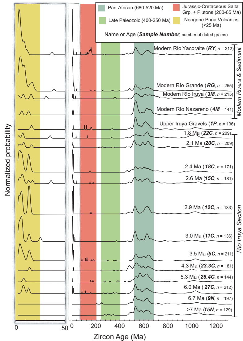
Fig. 8. Detrital zircon spectra from the Orán Group and modern rivers, including the Río Grande and Río Yacoraite from Streit et al. (2015). The Orán Group shows three major provenance shifts: 1) the appearance of Jurassic–Neogene zircons at ca. 6.3 Ma, 2) the abundance of Neogene zircons from ca. 4.0–2.3 Ma, and 3) the decline in Neogene zircons after 2.3 Ma. Samples 11c and 12c show a pronounced ‘double hump’ Pan-African distribution similar to the modern Río Nazareno and Proterozoic–Paleozoic bedrock units displayed in Fig. 8. Neogene populations from the Río Iruya section show prominent 6–7 and 12–14 Ma peaks, most likely derived from the Panizos caldera and Pozuelos basin.
