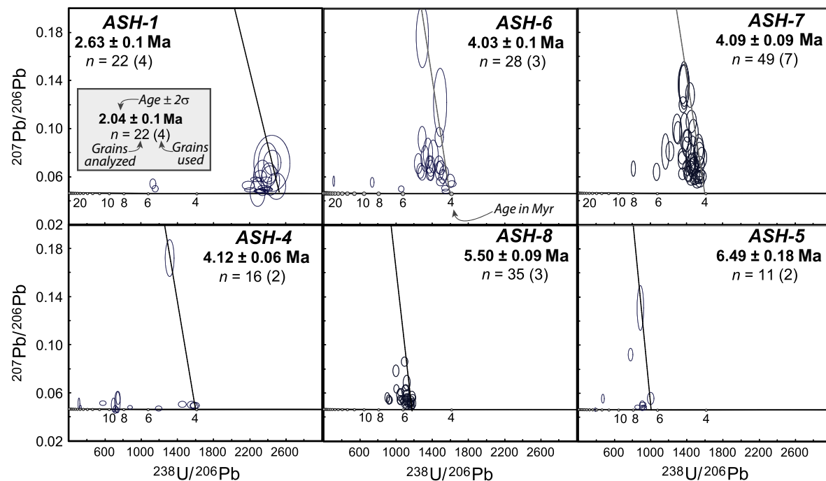
Fig. 5. Tera-Wasserburg concordia plots of LA-ICPMS U-Pb zircon data for the six tephra samples displayed as 2\sigma ellipses. Thin line represents the best-fit mixing line between an initial ^{207}\text{Pb}/^{206}\text{Pb} of 0.84 and the measured ratios of the youngest grains. Thick horizontal line is the concordia line with ages labelled in Ma. Preferred eruption ages are shown in bold, along with the # of grains dated ( n ) and the number used to estimate the preferred age (parentheses).
